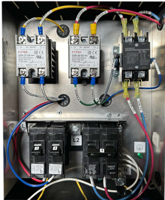
Figure 1.1 — Electrical Panel with Back Panel Removed
