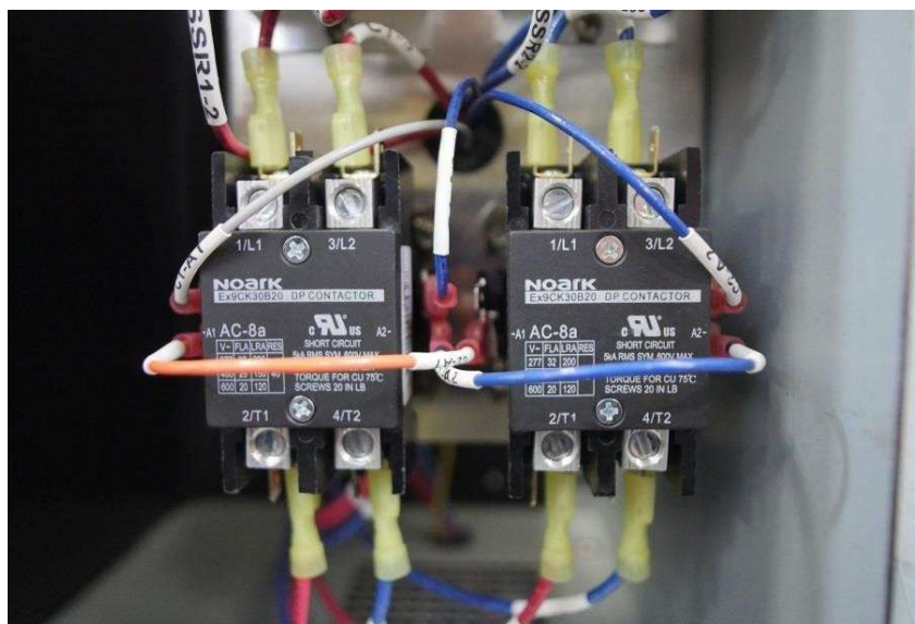
Noark Contactors
